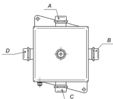
KM-O IP66-100x100
