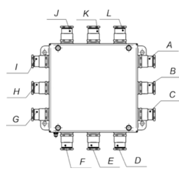
KM-B 2020 KM-BO 2020
