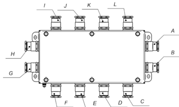
KM-B 1530 KM-BO 1530
